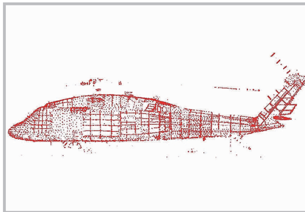
Fig. 4: External skin panels - Scan data established by TRITOP (photogrammetry) (9,000 points, accuracy of 0.1 mm, object size > 15 m)
